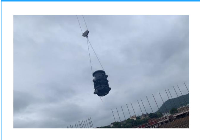
Tank hoisting
